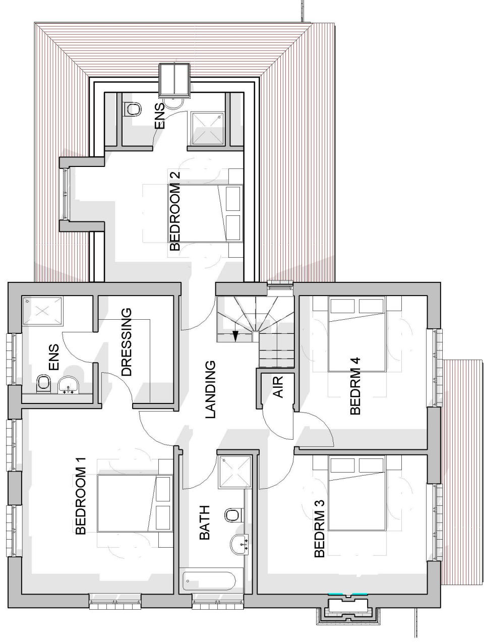
Plot 2 - First Floor Plan as Proposed 1 : 100
