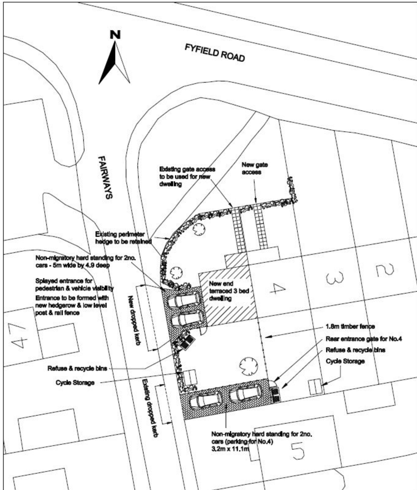
Site Layout Details
