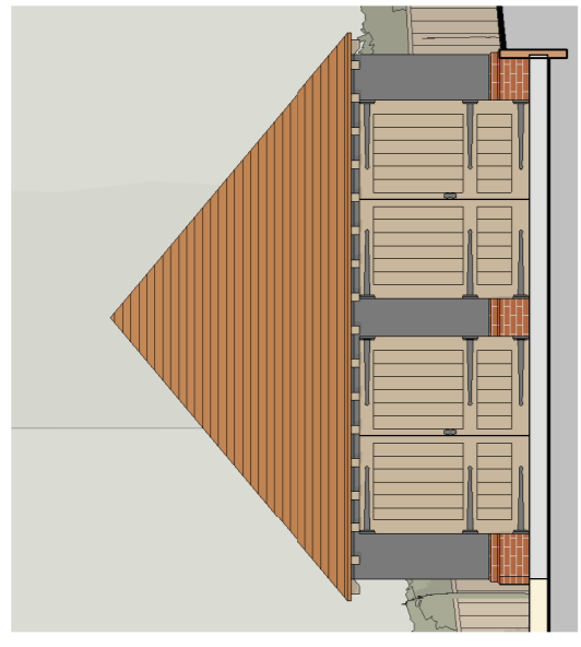
Garage 2 - East Elevation 1:100
