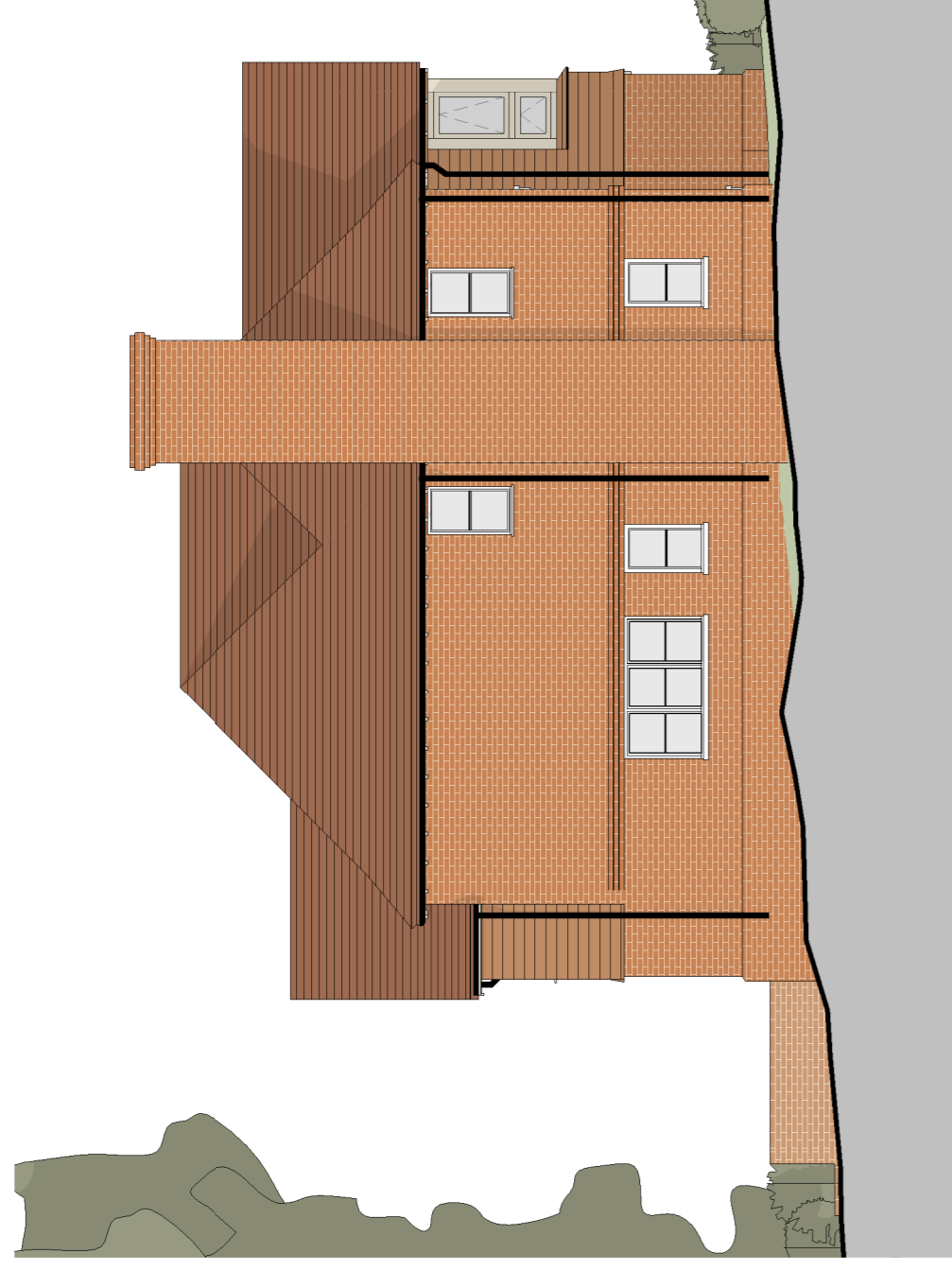
House 2 - East Elevation 1:100
