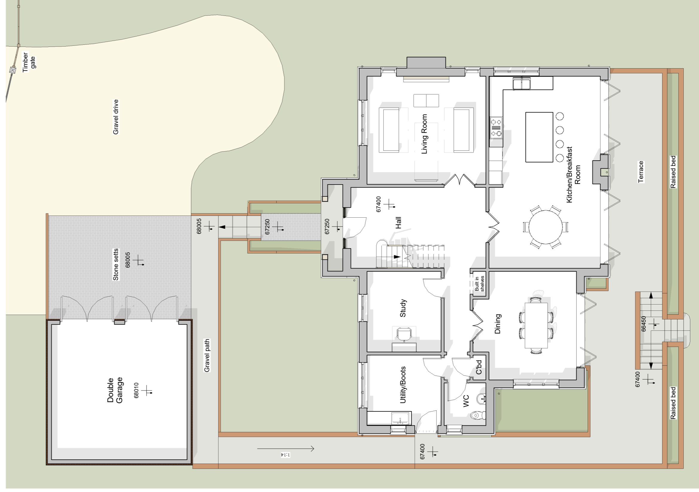
House 2 - Ground Floor Plan 1:100
