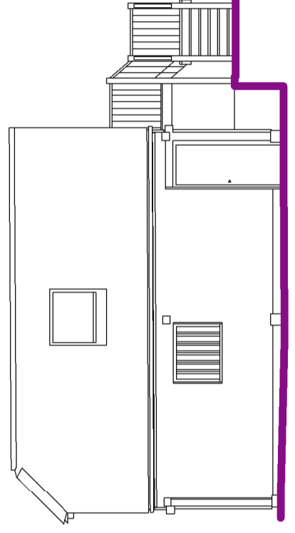
Garage - East Elevation as Existing 1 : 100
