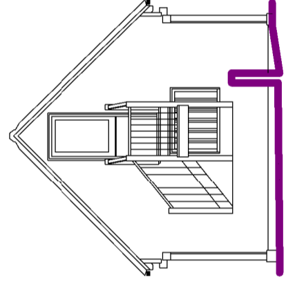
Garage - North Elevation as Existing 1 : 100
