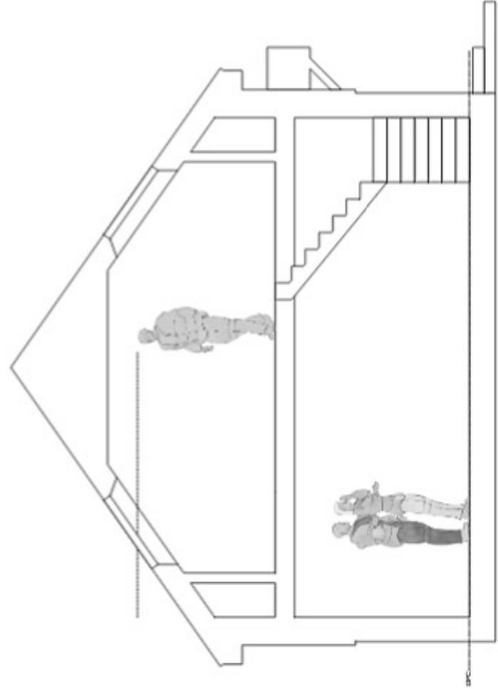
8 SECTION SCALE 1:50
