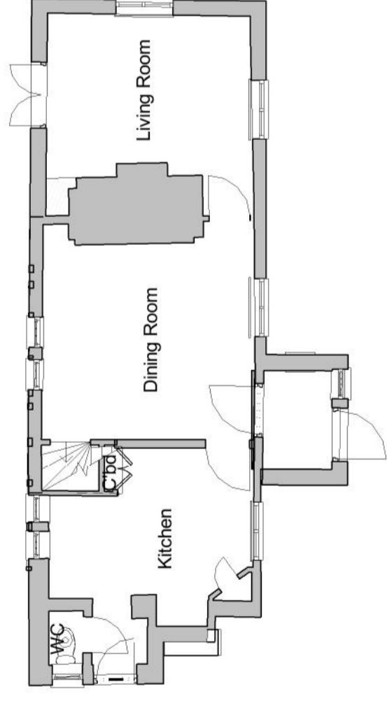
Ground Floor Plan as Existing 1 : 100
