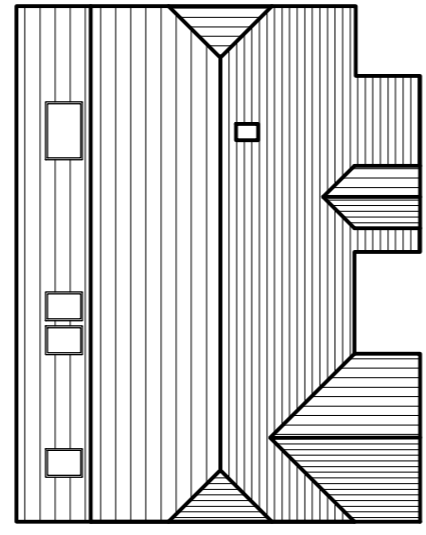
PROPOSED ROOF PLAN 1:200
