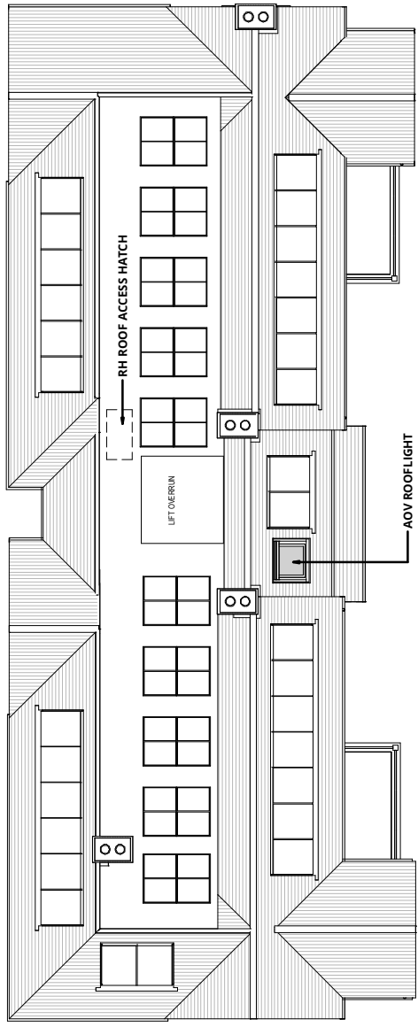
ROOF PLAN
