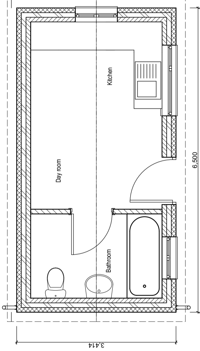
Utility/Day Room - Indicative layout
