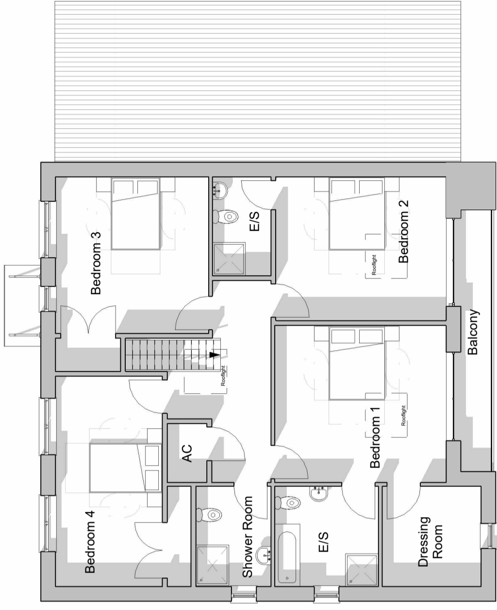
Proposed First Floor Plan 1 : 100
